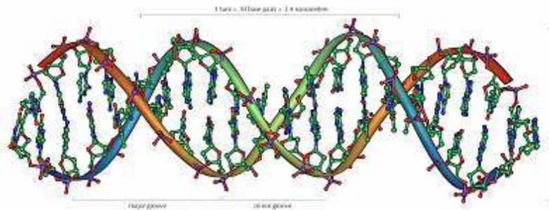
Figure #3 A drawing of an X-ray crystallography of DNA showing the helical structure.
