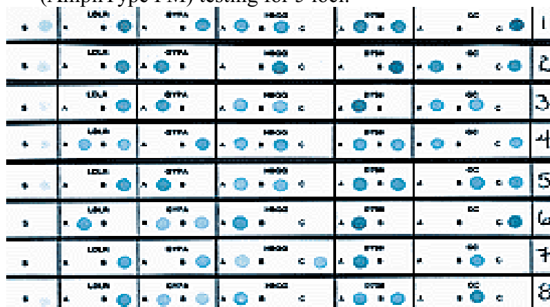
Figure #12. An example of the multiplex version (AmpliType PM) testing for 5 loci. 59
