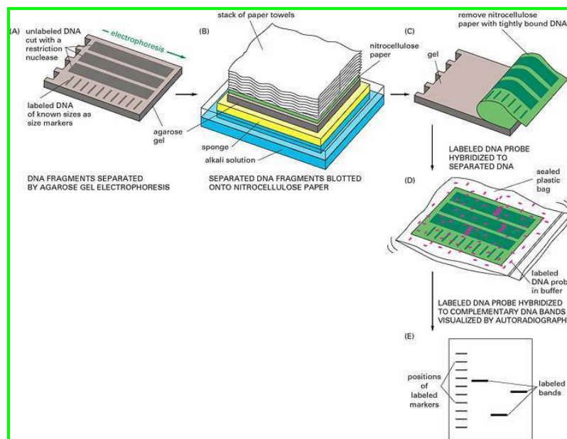
Figure #7. The Southern Blot Technique.
