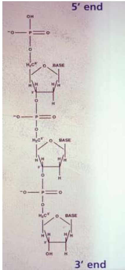
Figure #4 Deoxyribose with the 3' and 5' binding sites identified.
