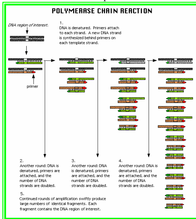
Figure #6 The principle of PCR. By using techniques to increase the number of DNA molecules of interest, one strand of DNA can be multiplied millions of times.
