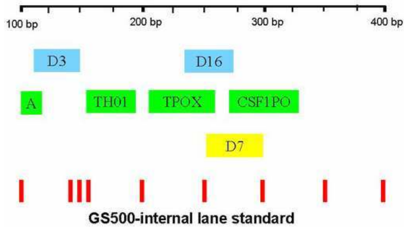
Figure #10 Example of a typical banding pattern seen with multiple fluorochrome dyes on a DNA specimen.
